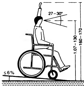
⑤ Wheelchair on a slope
